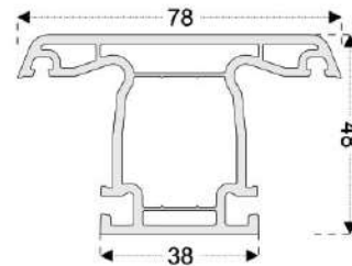
Mullion Profile
