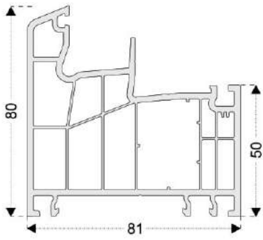
Frame Profile
