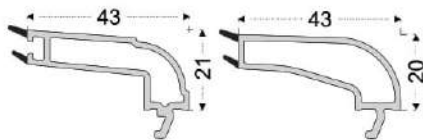
4-6 mm Single Glass G.Bead
