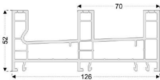
Triple Sliding Frame Profile
