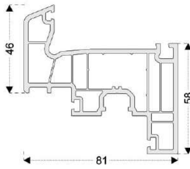
Sash Profile
