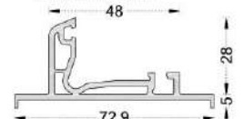
Mullion Profile
