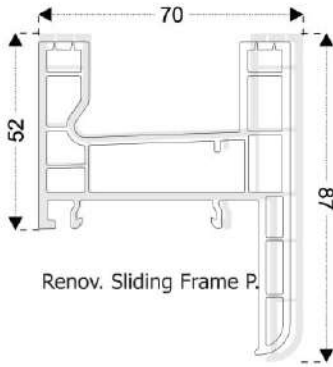
Renovation Sliding Frame P. with Flynet
