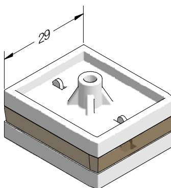
Mullion sealing block 96 MD SYNEGO®
