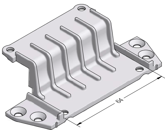
Mechanical connector muntin 124 MD SYNEGO® cross joint
