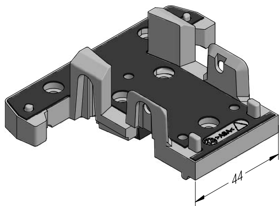
Mullion threshold support 96 SYNEGO®
