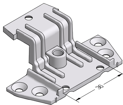
Mechanical mullion connector 96 MD SYNEGO® cross joint
