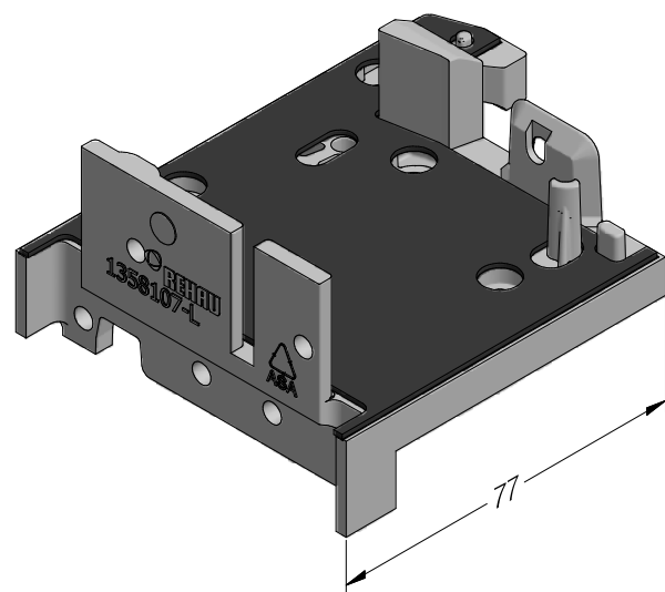
Frame threshold support 103 SYNEGO®
