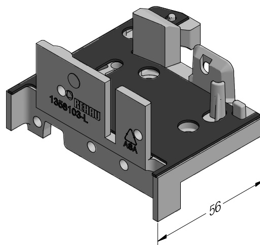
Frame threshold support 82 SYNEGO®
