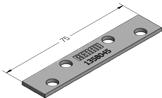
Mullion mounting plate 96 and 124 SYNEGO®
