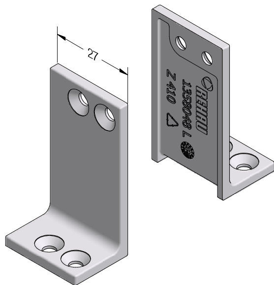
Set mullion brackets mullion cross joint MD SYNEGO®
