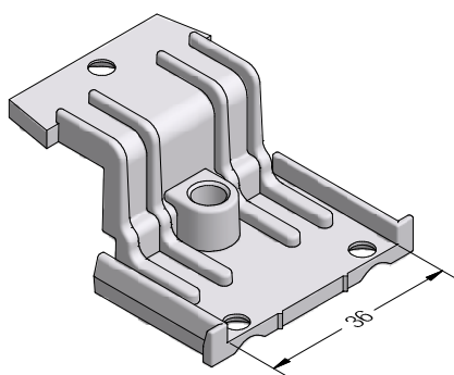
Mechanical mullion connector 96 MD SYNEGO®
