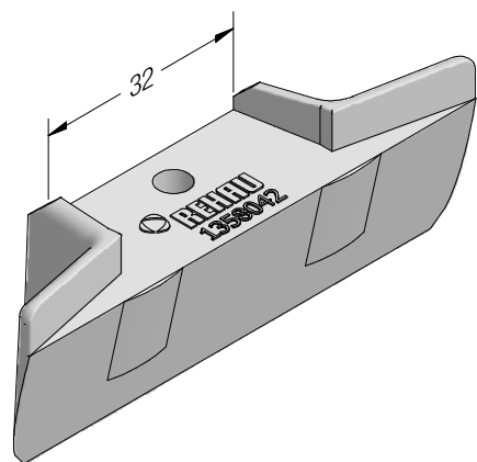
Mullion sealing block 96 MD SYNEGO®
