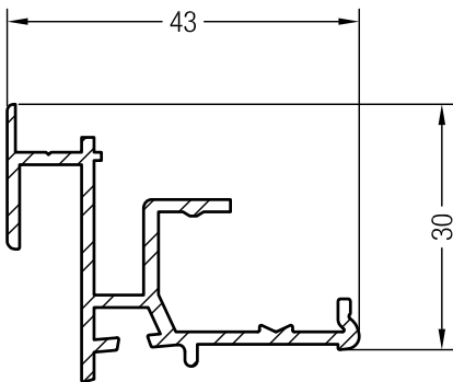
Compensating profile SYNEGO®
