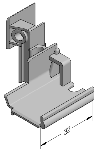
Compensating profile end cap®
