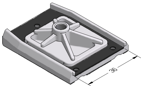
Mechanical mullion connector 96 AD SYNEGO®
